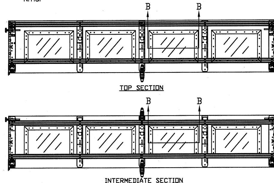
OPTIONAL SHORT PANEL GLAZED SECTION STRUT AND STILE LAYOUTS N.T.S.
